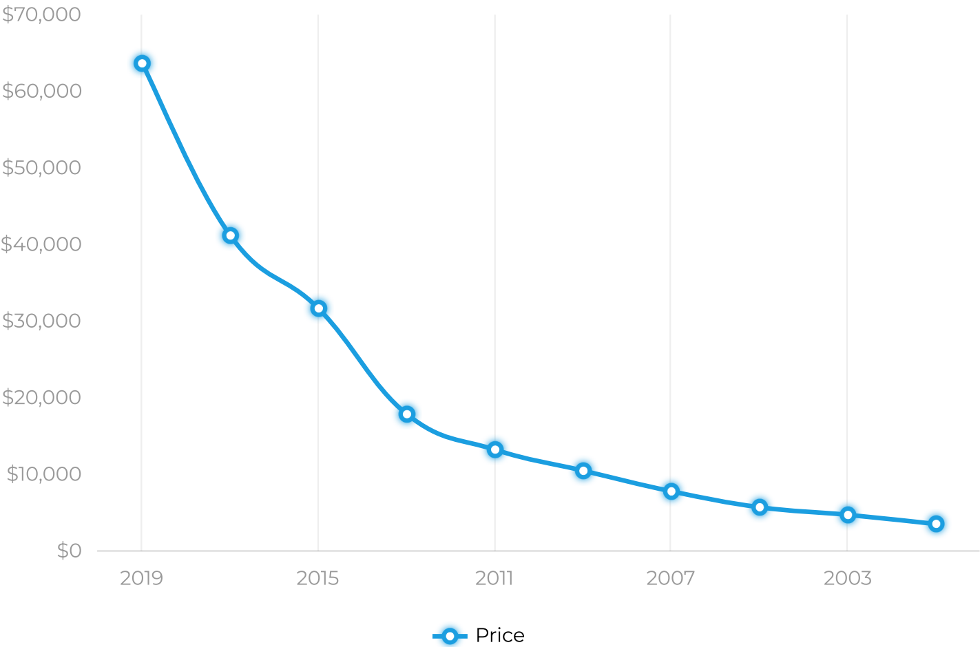
Price/Year Dependence
